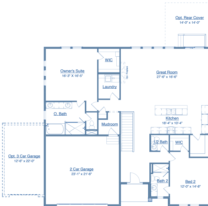
MAIN LEVEL
