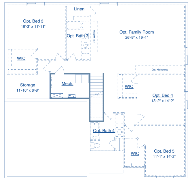
LOWER LEVEL
