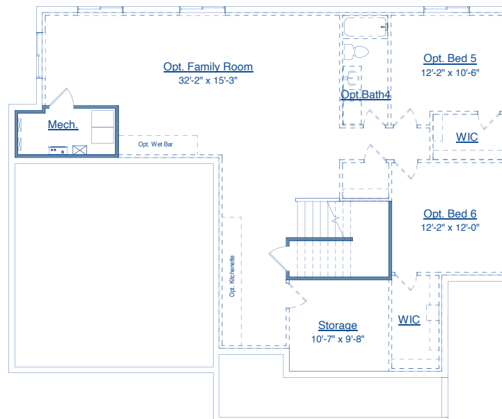
LOWER LEVEL
