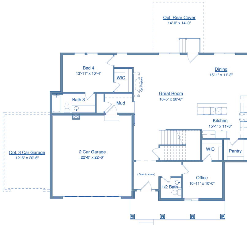
MAIN LEVEL
